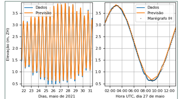
Comparison between data and OPENCoastS predictions
